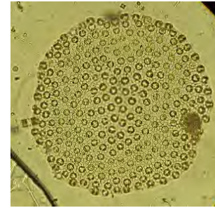
Planktoniella muriformis consorcio discoide
